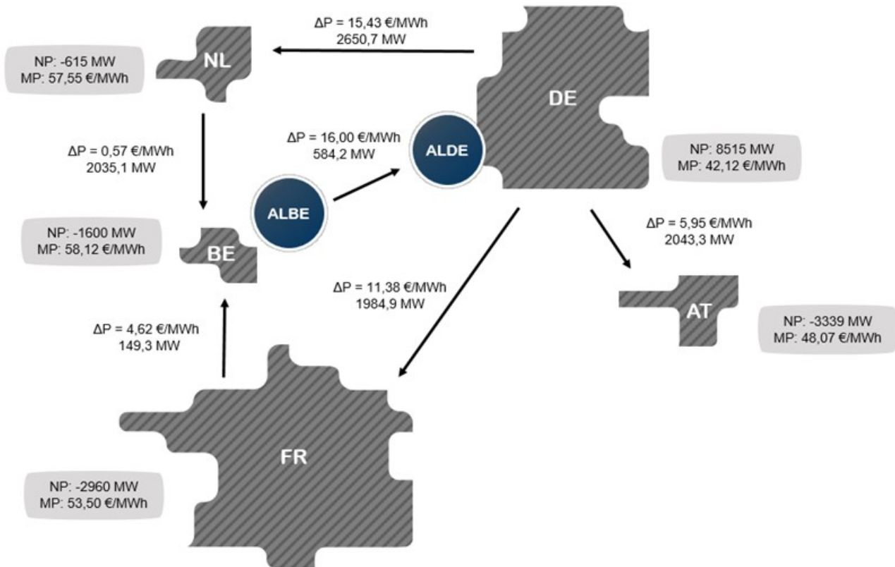
Figure 2: The calculated additional aggregated flows, based on the PTFs and net positions.
